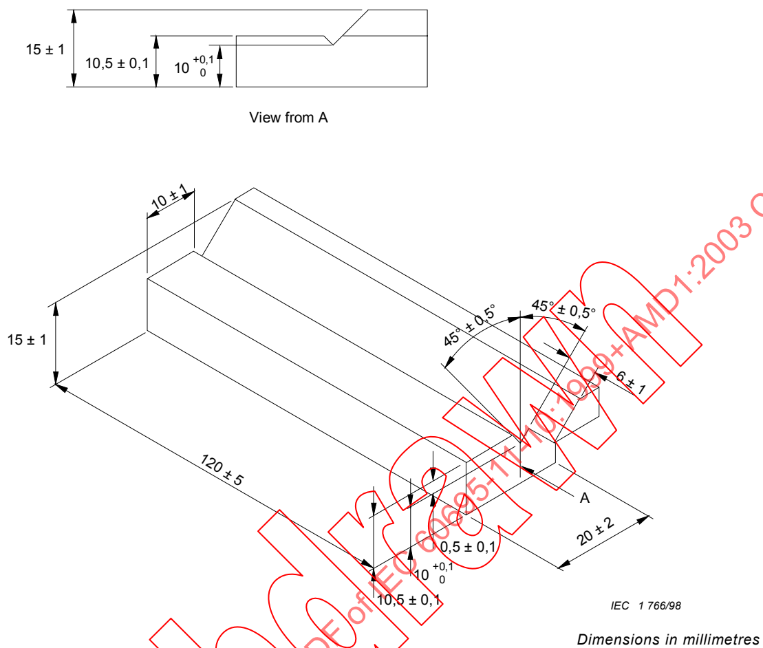
Figure 2 – Flexible specimen support fixture – method A
