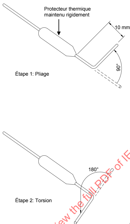
Figure 1 – Essai de torsion
