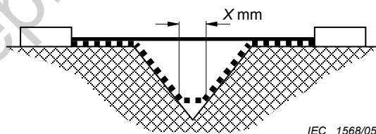
Figure AA.2 – Wide groove
