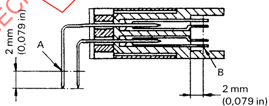
Figure 37 — Connection points for contact resistance measurements
