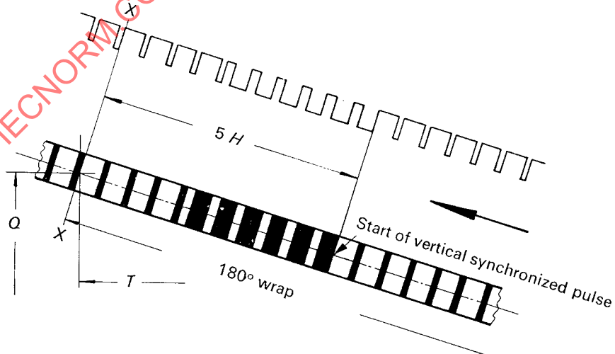
Detail b: End of recorded video track (NTSC).
