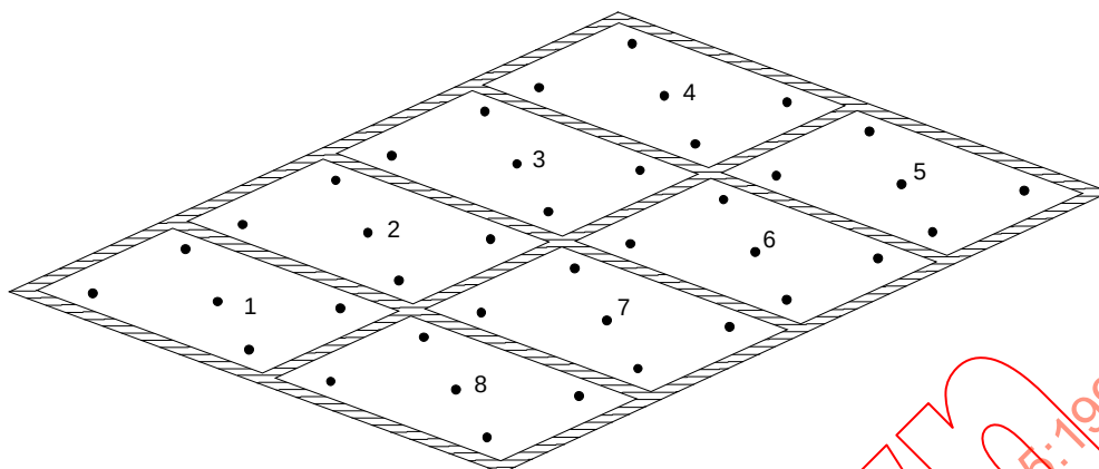
Figure 101a – Positioning of temperature sensors on the contact surface of the heated area of a HEATING DEVICE (see 2.12.101, 50.101 and 50.105)
