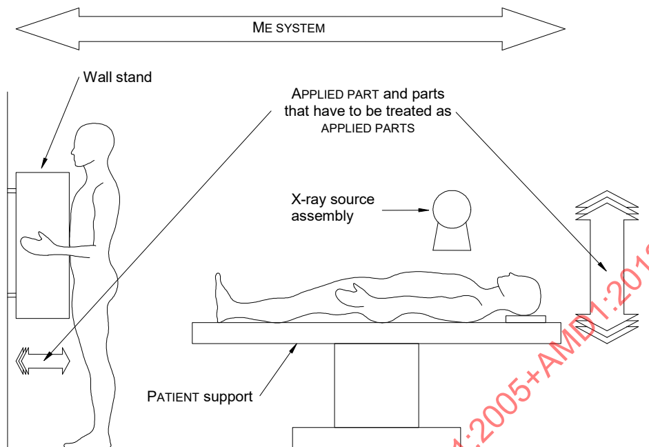
Figure A.5 – Identification of APPLIED PARTS and PATIENT CONNECTIONS in an X-ray ME SYSTEM
