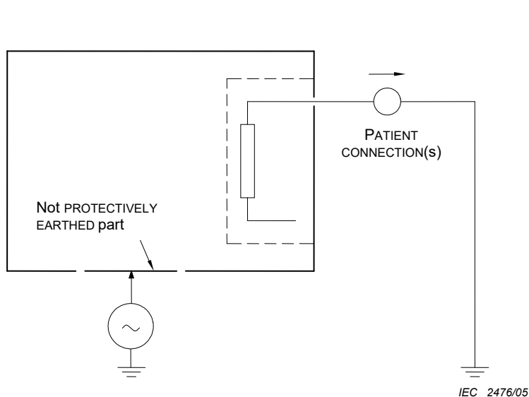
Figure K.5 – ME EQUIPMENT with a PATIENT CONNECTION of a TYPE BF APPLIED PART that is not PROTECTIVELY EARTHED (simplified Figure 18) (see 8.7.4.7 d))
