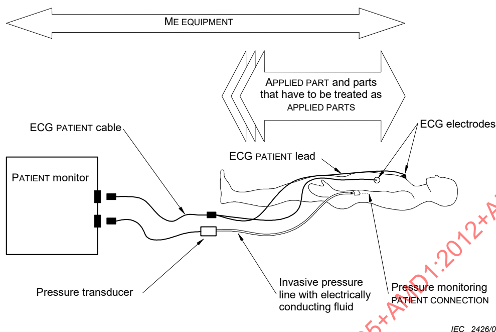
Figure A.4 – Identification of ME EQUIPMENT, APPLIED PARTS and PATIENT CONNECTIONS in a multifunction PATIENT monitor with invasive pressure monitoring facilities
