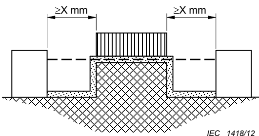
Figure 28 – CREEPAGE DISTANCE and AIR CLEARANCE – Example 7
