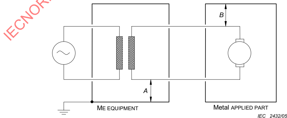
Figure A.10 – Floating circuit
