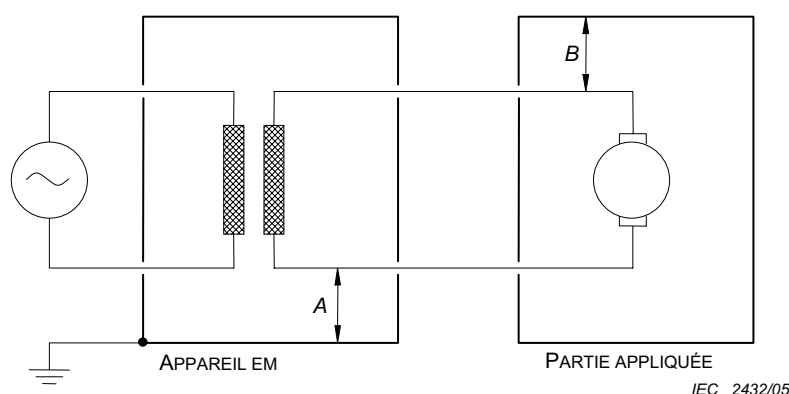
Figure A.10 – Circuit flottant
