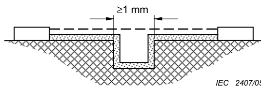
Figure 24 – CREEPAGE DISTANCE and AIR CLEARANCE – Example 3
