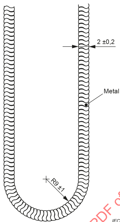
Figure 35 – Test chain
