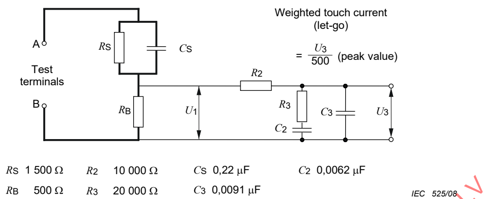
Figure G.3 – Measuring network, touch current weighted for let-go (for portable class I luminaires)
