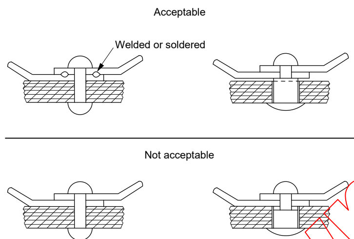
Figure 17 – Construction of electrical connections
