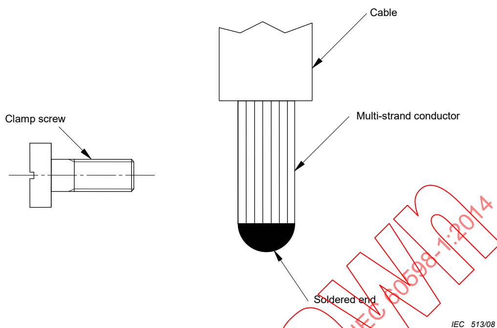
Figure 28 – Example of permitted degree of soldering
