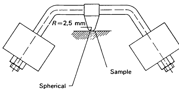
Figure 10 – Ball-pressure apparatus
