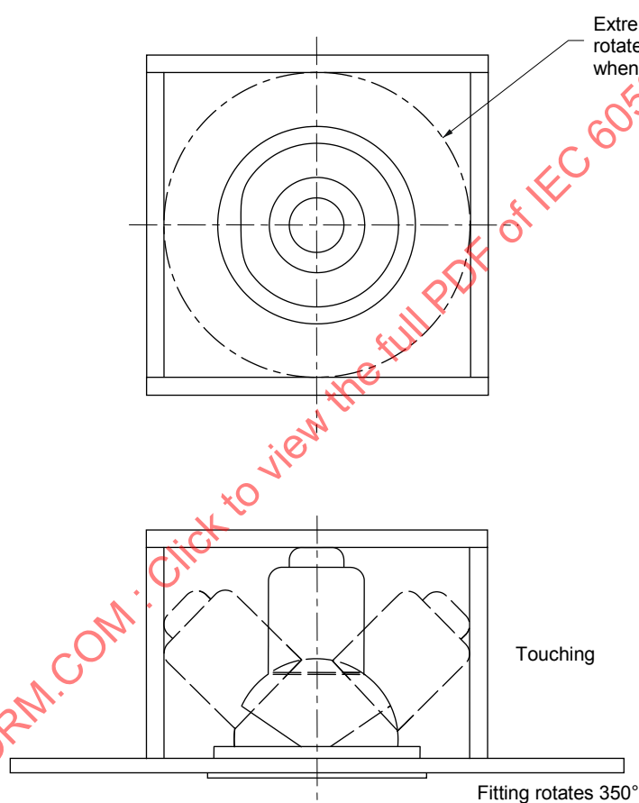
Figure D.2 – Correct test box size (insulating ceilings) for settable and adjustable luminaires
