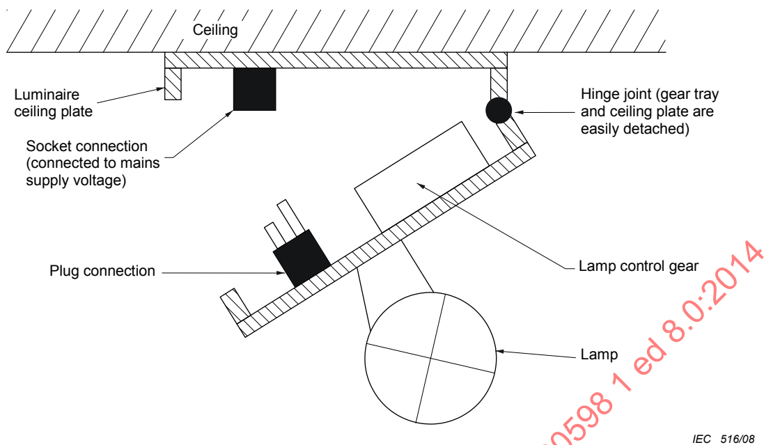
Figure 31 – Electro-mechanical contact system with plug/socket connection
