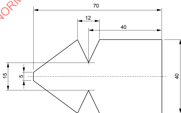
Figure 8 – Mounting support
