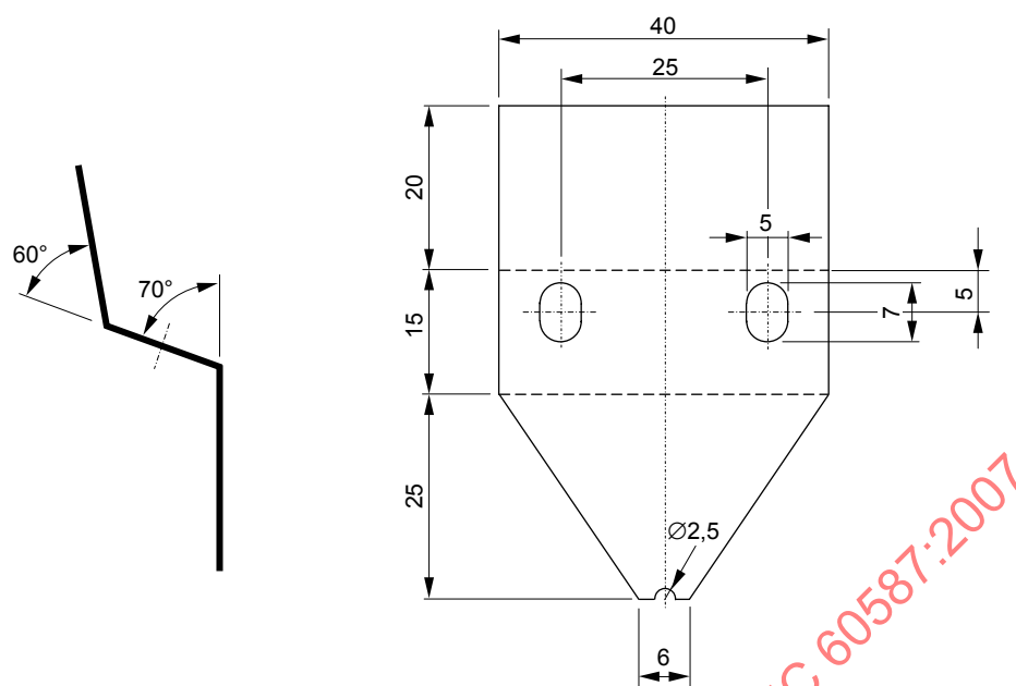
Figure 4 – Top electrode, stainless steel 0,5 mm thick
