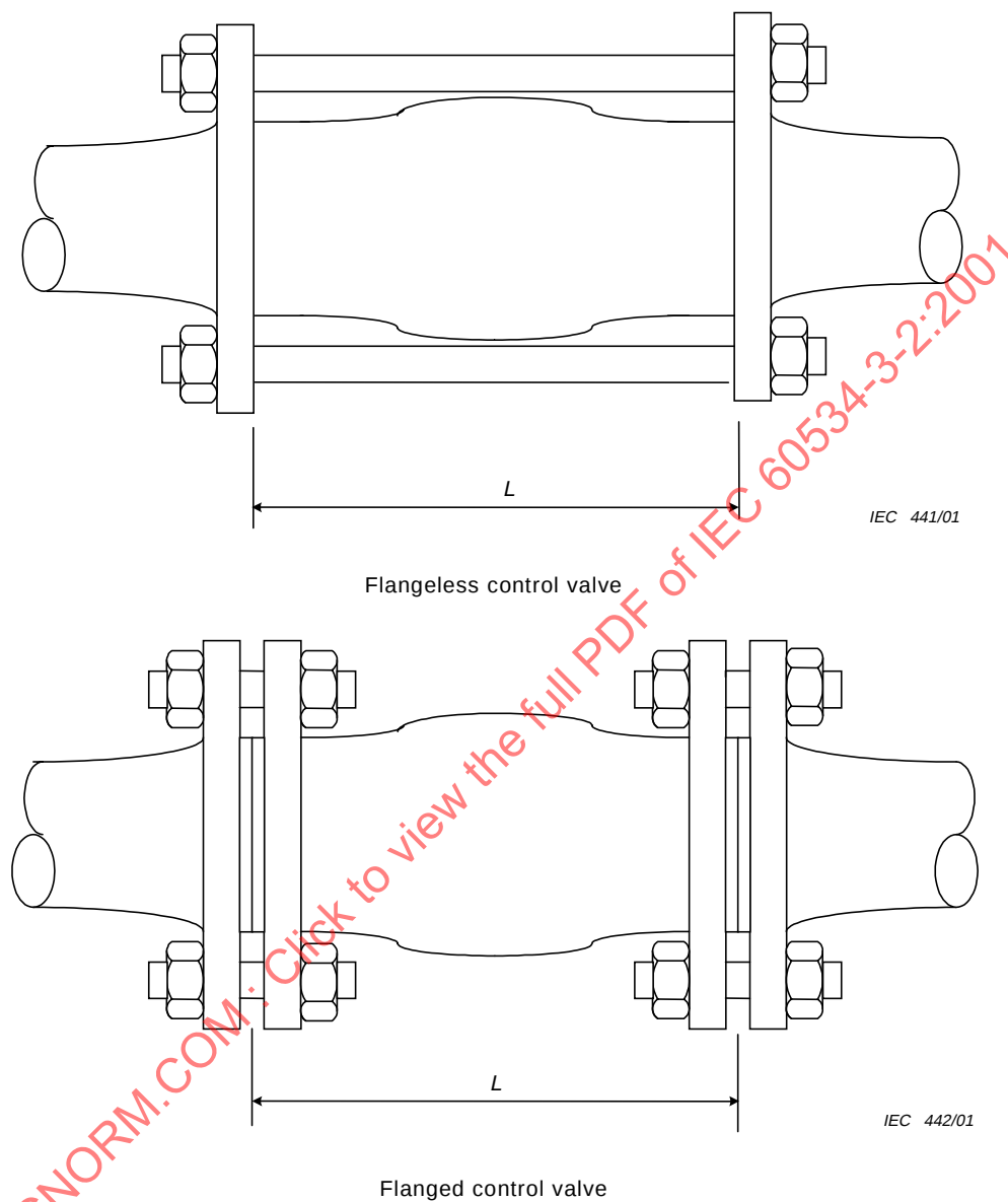
Figure 1 – Face-to-face dimensions
