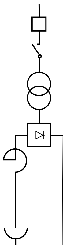
Figure AA.4 – DC furnace supply with HV furnace switch (or HV furnace breaker) in open position and HV disconnect in open position
