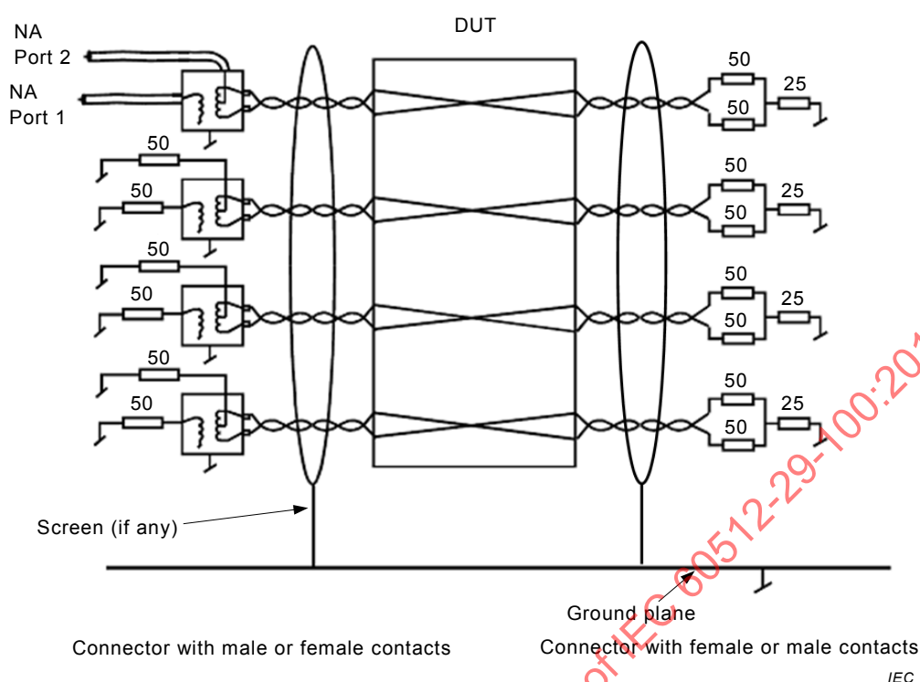
Figure 19 – TCL measurement
