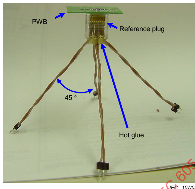
Figure 24 – Reference FEXT plug-test lead position
