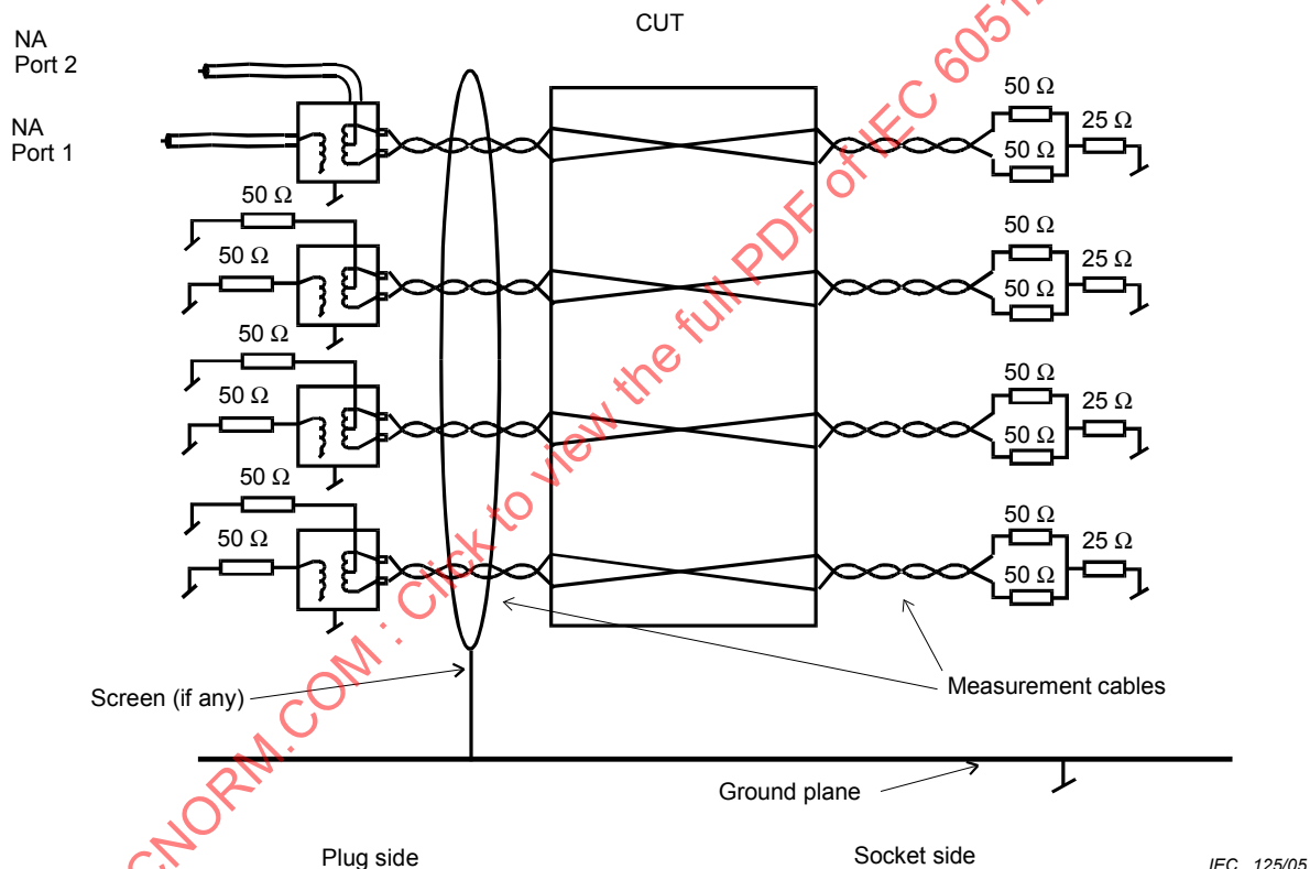
Figure 15 – TCL measurement
