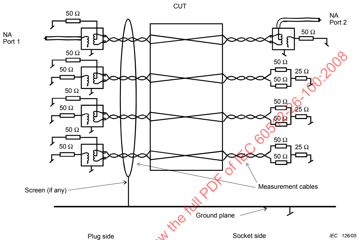
Figure 16 – TCTL measurement
