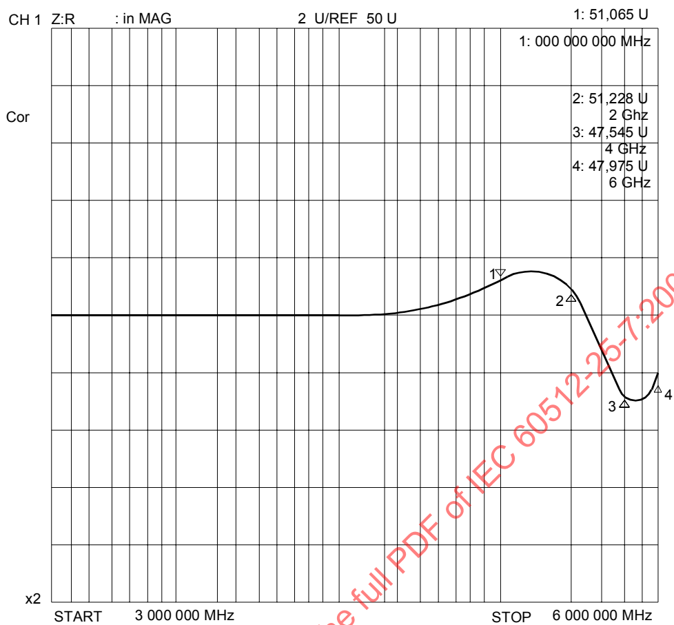
Figure A.3 – Example of analyzer output, impedance versus log frequency plot
