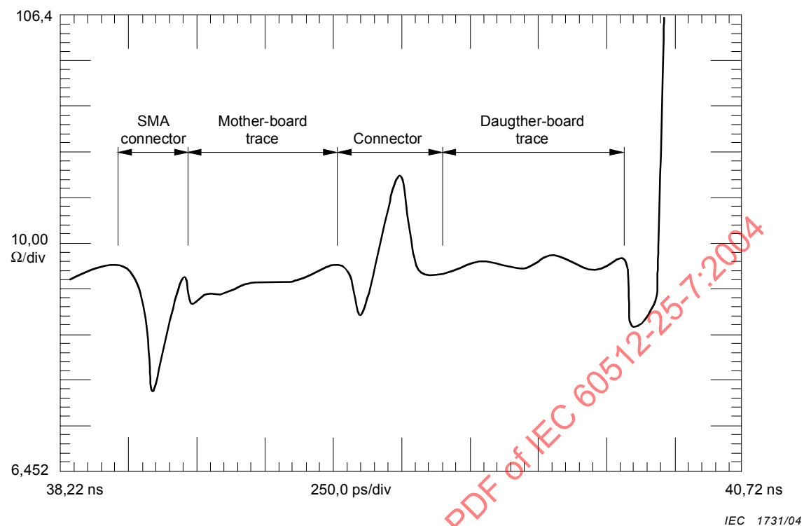
Figure D.1 – Example of an impedance profile of connector using a measurement system rise time of 35 ps
