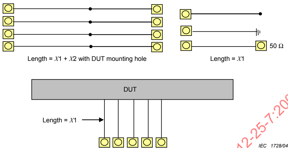
Figure C.1 – Typical mother-board test fixture
