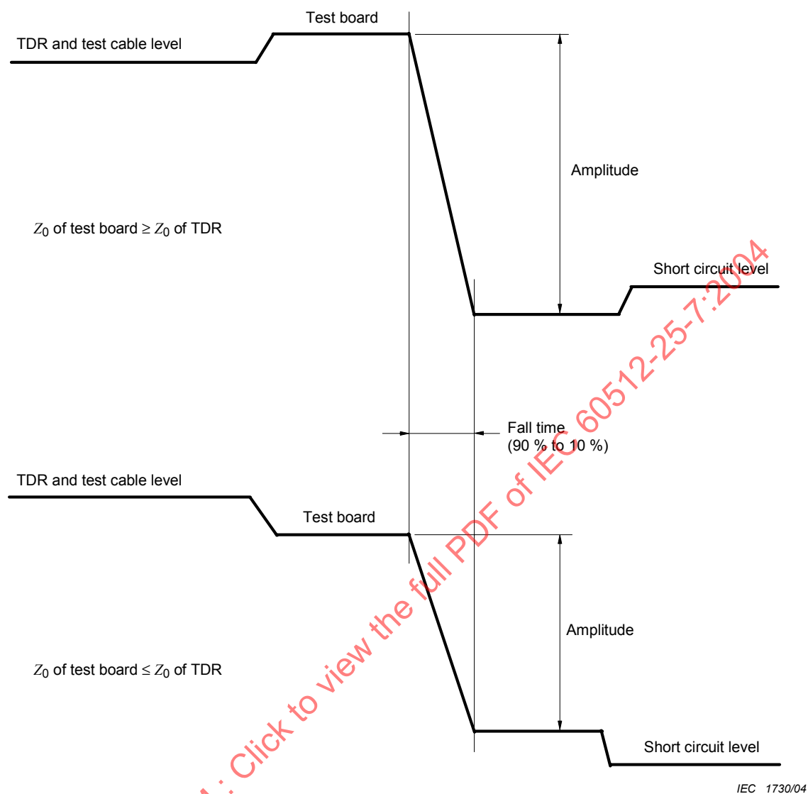
Figure C.3 – Example of near-end reference trace
