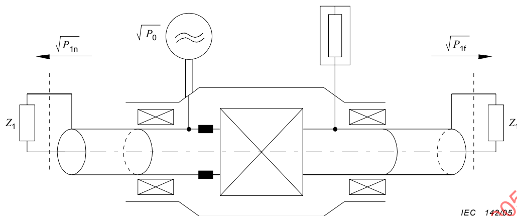
Figure 5 – Schematic measurement circuit
