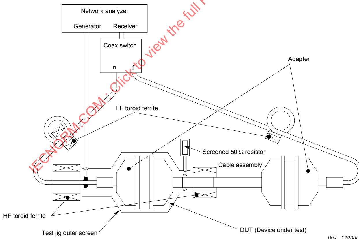
Figure 3 – Example of a practical measurement set-up
