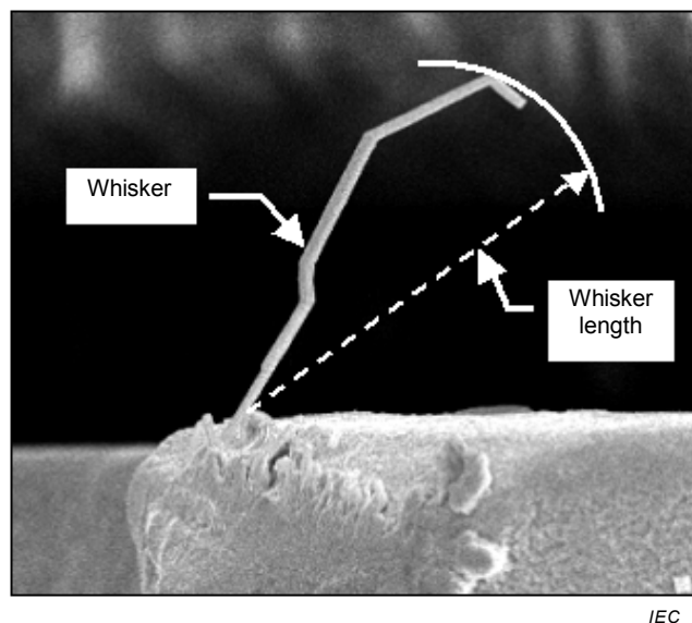
Figure 1 – Whisker length
