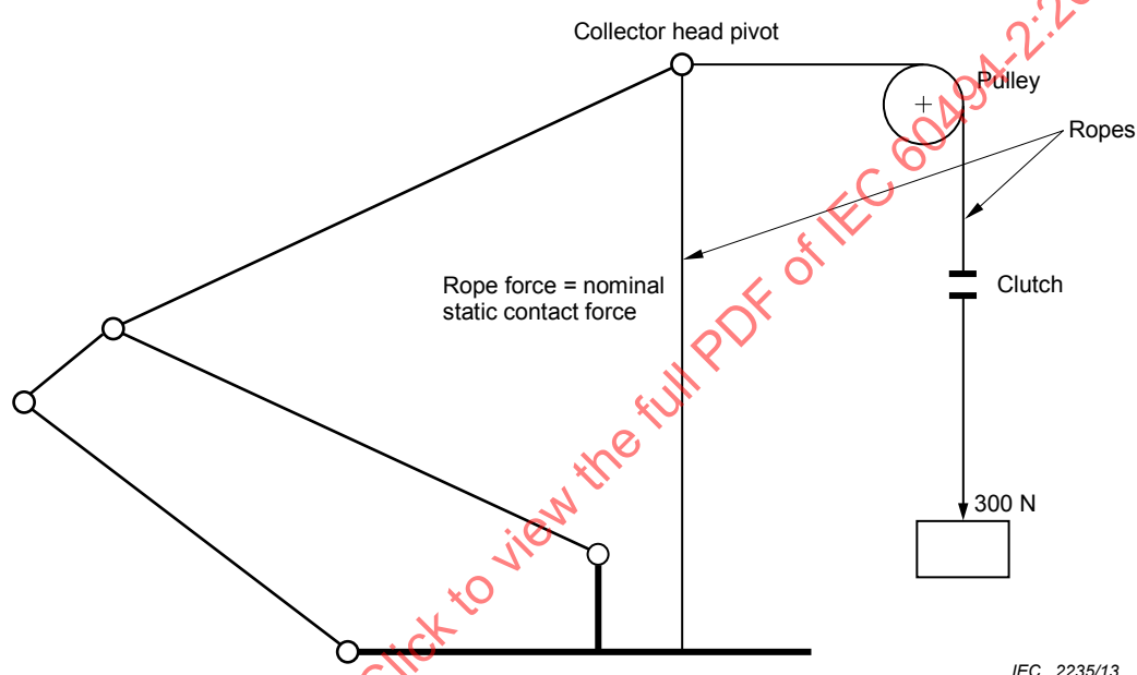
Figure 2 – Test principle
