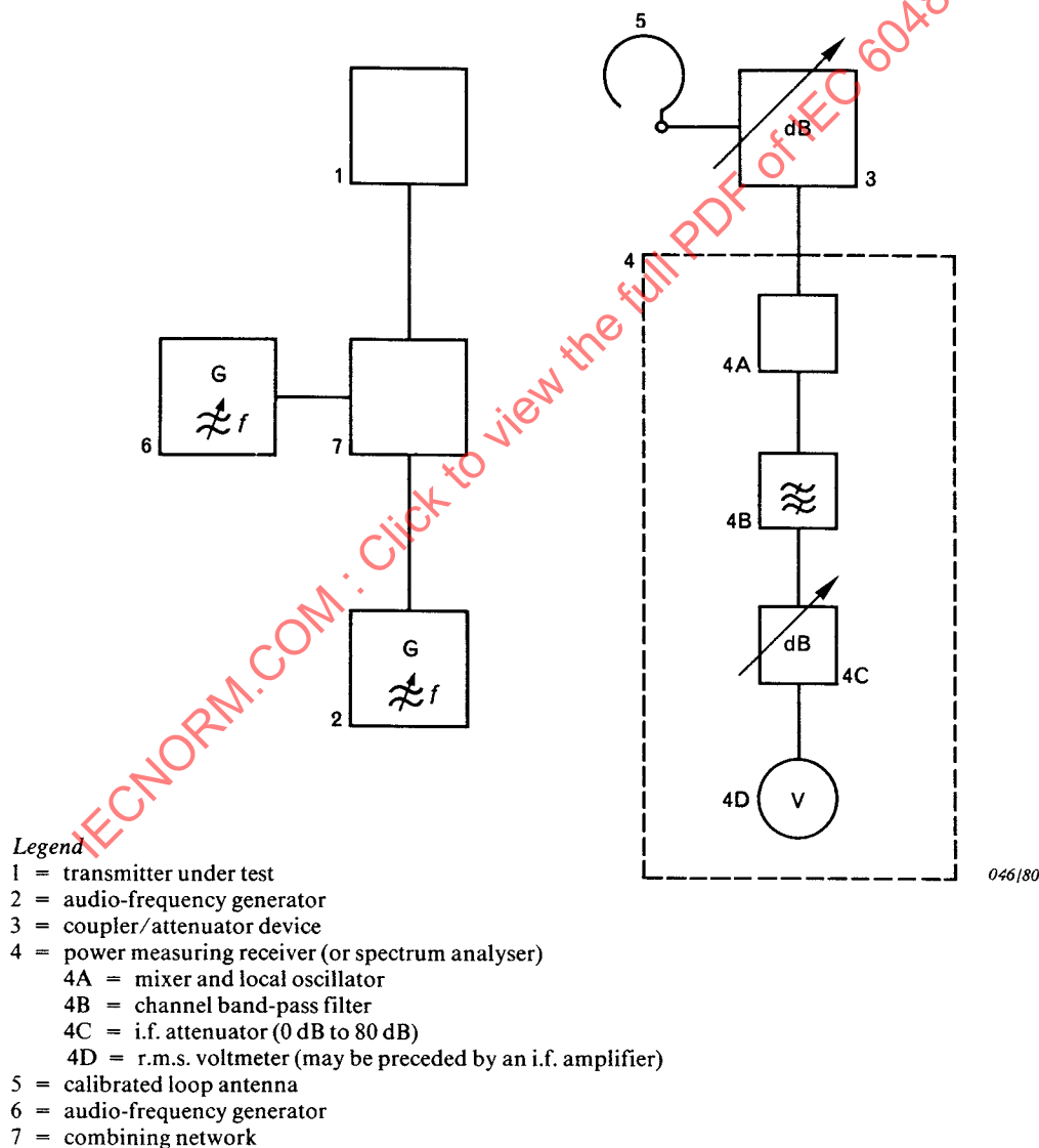
FIG. 7. — Measuring arrangement for radiated adjacent channel power.
