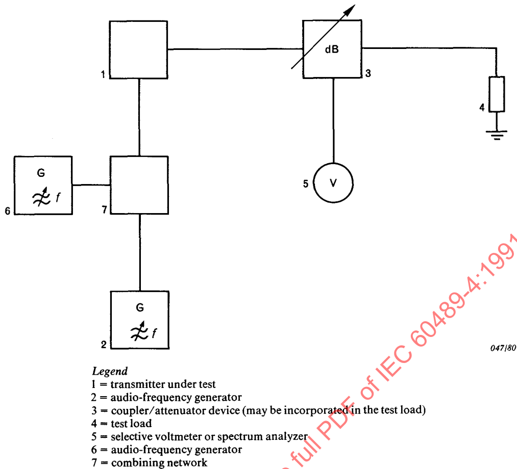
FIG. 9. — Measuring arrangement of transmitter characteristics.
