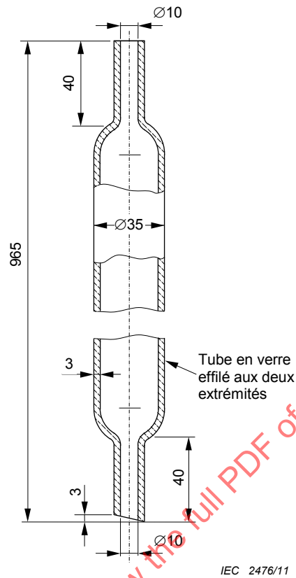
Figure 3 – Pipette
