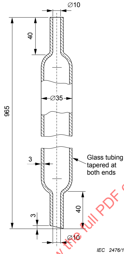
Figure 3 – Pipette
