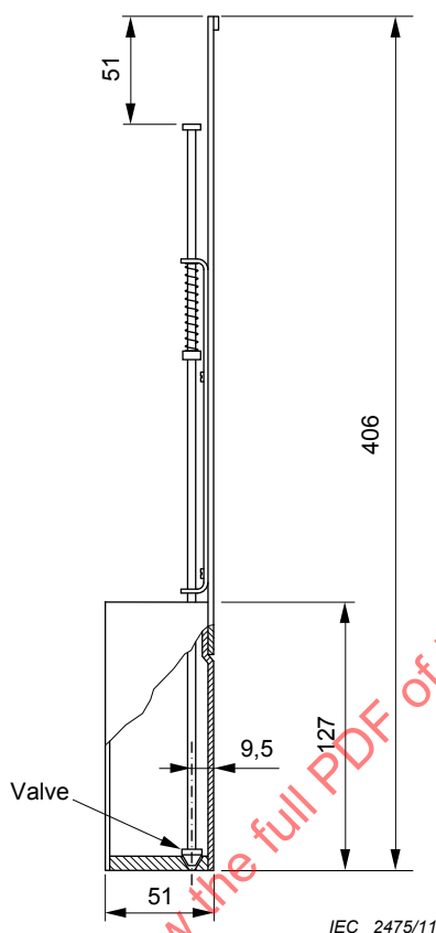
Figure 2 – Cream dipper
