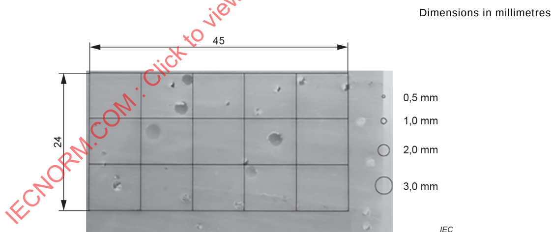
Figure A.2 – Position of examination grid on the specimen
