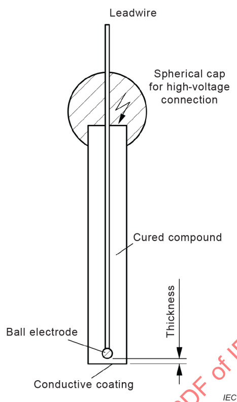
Figure 4 – Example of electrode arrangement for rigid cured compound
