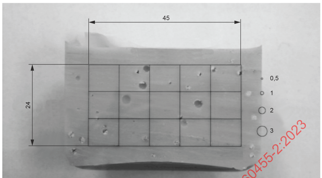
Figure 2 – Position of examination grid on the specimen
