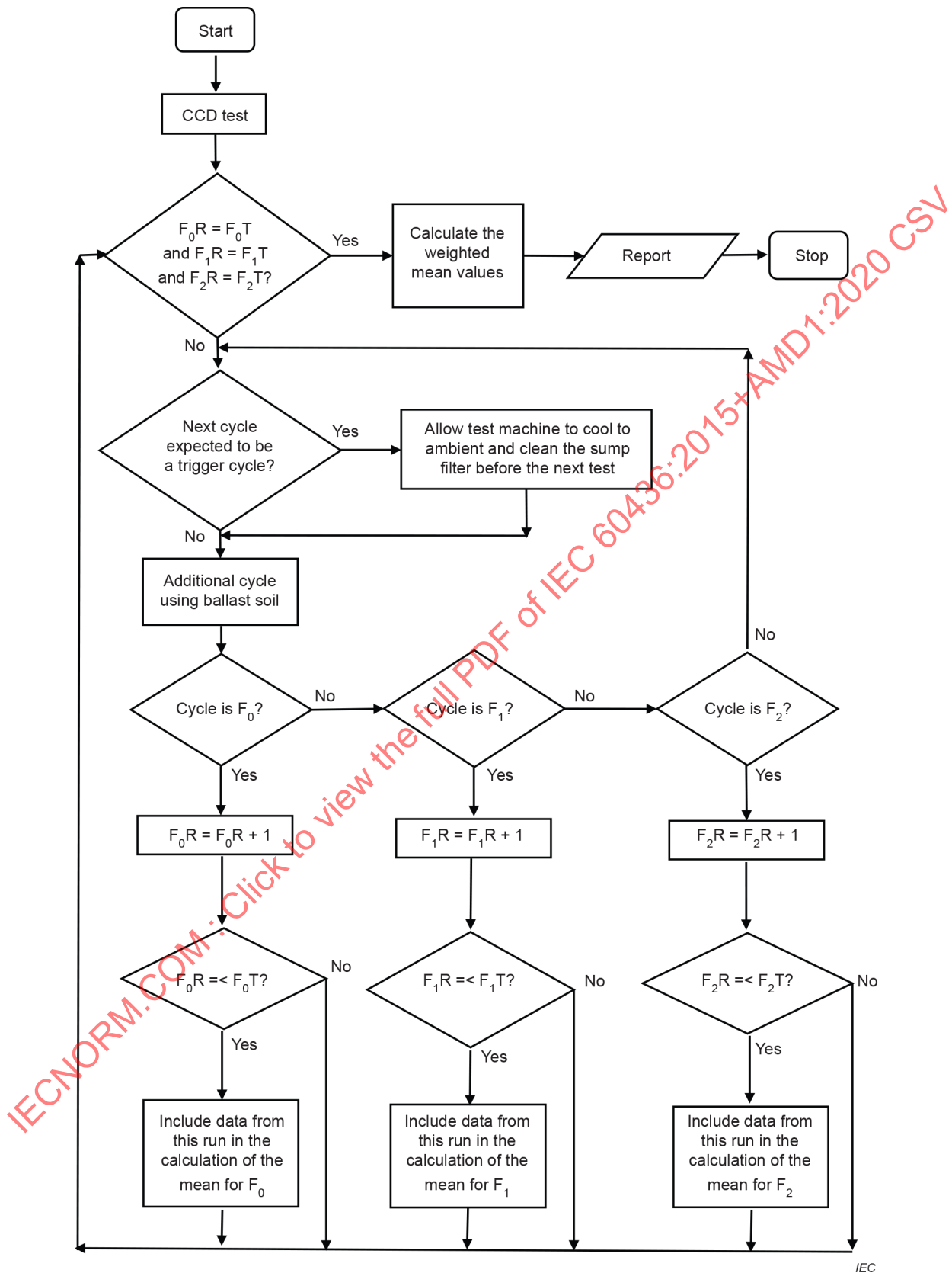
Figure V.1 – Flow chart showing the general test design for assessing intermittently recurring functions
