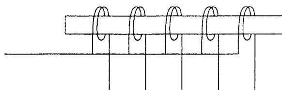
Figure 3 – Diagram of the connections of the five coils of the primary winding
