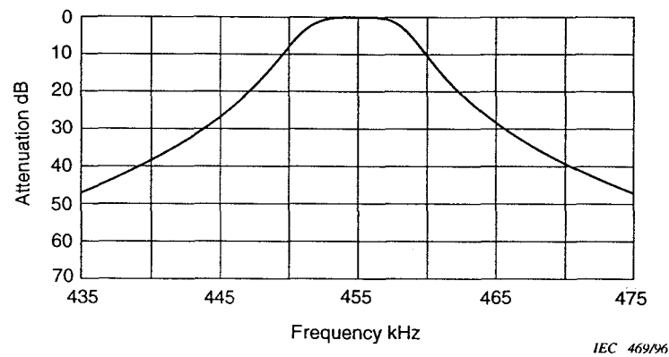
Figure 7a – Example of transducer amplitude of a piezoelectric ceramic filter using resonators with electrodes split into ring and dot
