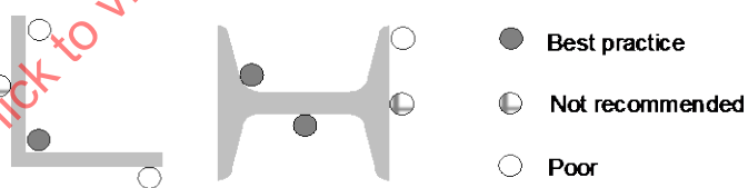
Figure 44.R21 – Location of cables inside metallic construction elements
