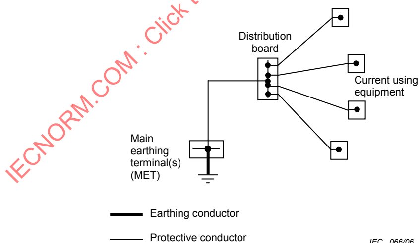
Figure 44.R13 – Examples of protective conductors in star network
