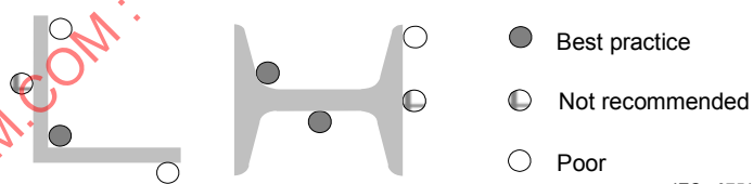
Figure 44.R21 – Location of cables inside metallic construction elements
