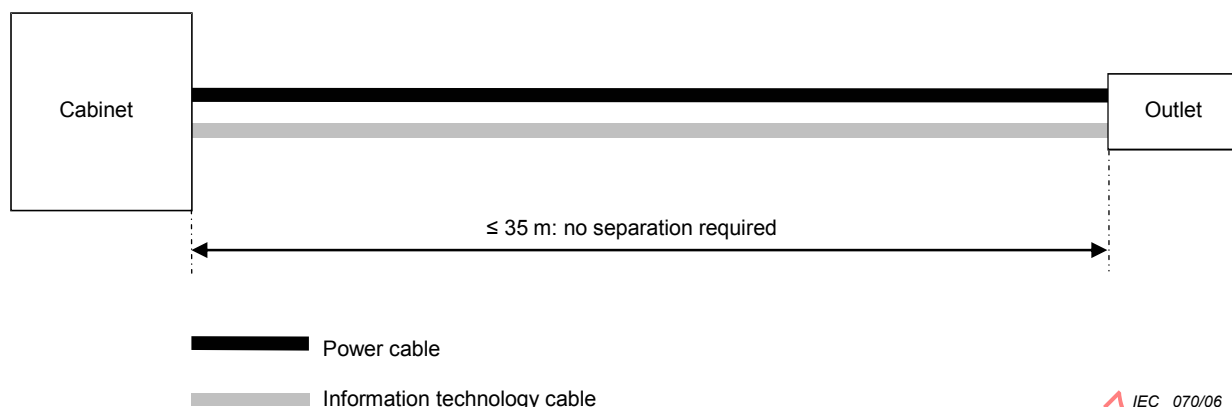
Figure 44.R17A – Separation between power and information technology cables for cable route lengths \leq 35 m
