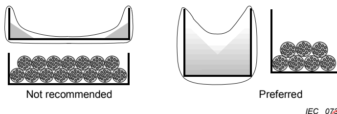
Figure 44.R19 – Cable arrangements in metal cable-trays
