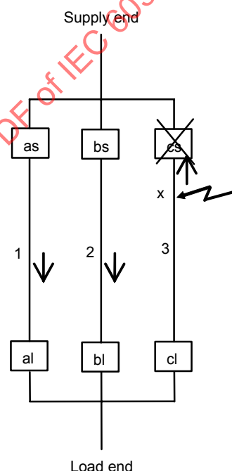
Figure A.4 – Current flow after operation of the protective device cs
