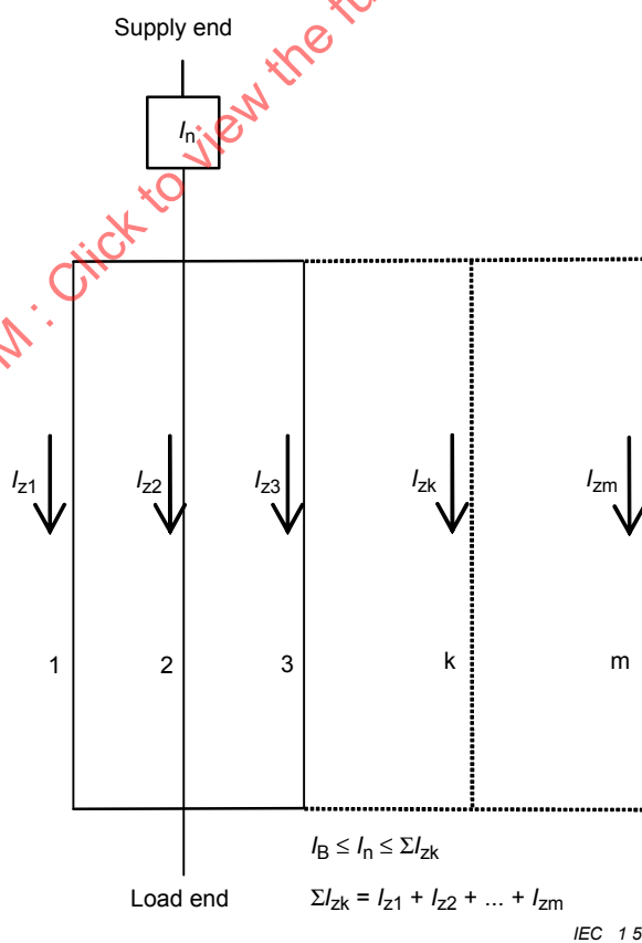
Figure A.2 – Circuit in which a single overload protective device is provided for the m conductors in parallel
