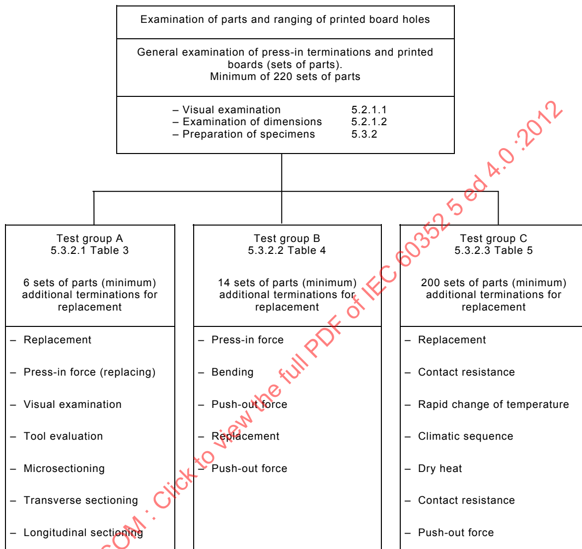
Figure 9 – Qualification test schedule
