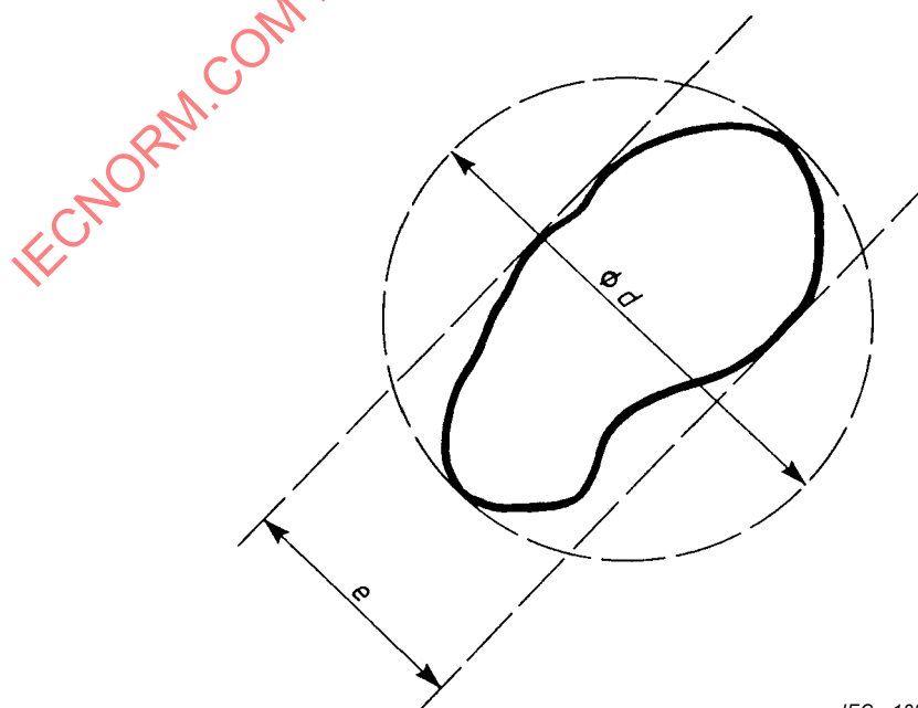
Figure AA.1 – Determination of standard aperture
