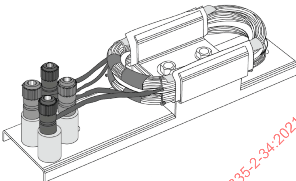
Figure BB.2 – Completely assembled motorette
