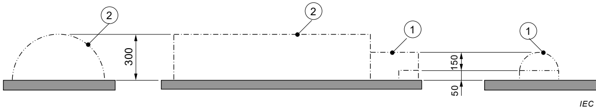
Figure 101 – Measuring points for appliances that are arranged over a person
