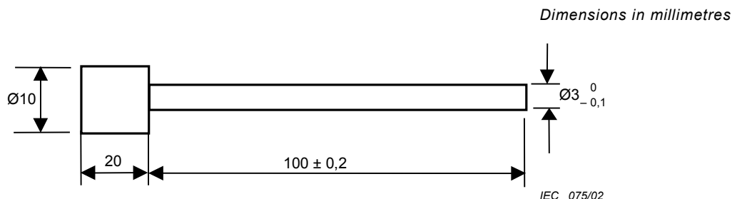
Figure 101 – Test rod for interlock concealment
