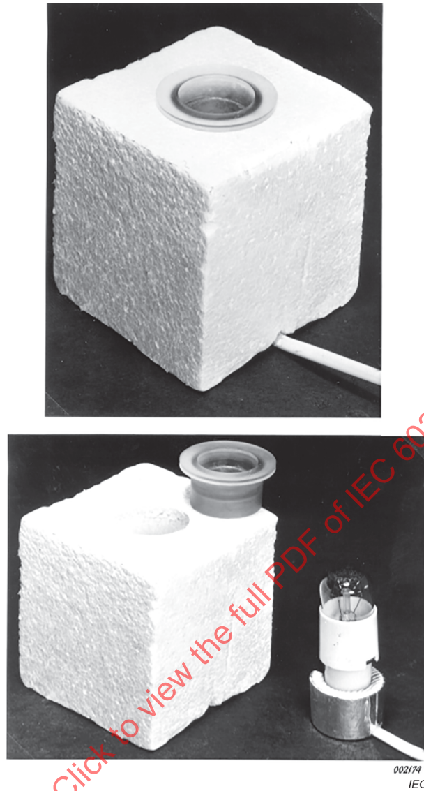
Figure BB.2 – Apparatus for water evaporation and for accumulation of frost
