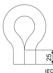
Figure 103 – Configuration of the hose for the freezing treatment
