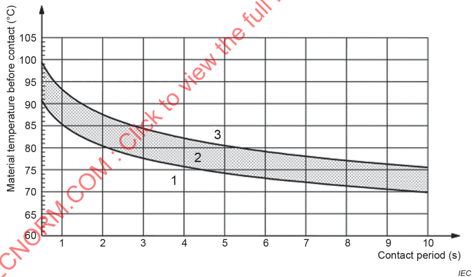
Figure 103 – Burn threshold spread when the skin is in contact with a hot smooth surface made of ceramics, glass and stone materials
