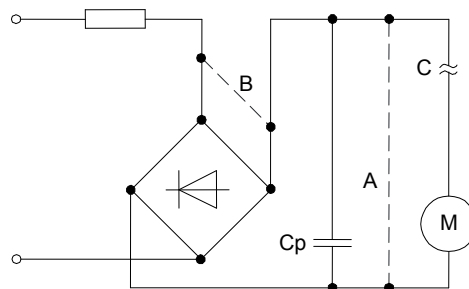
Series circuit
