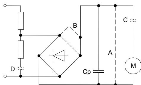
Parallel circuit
