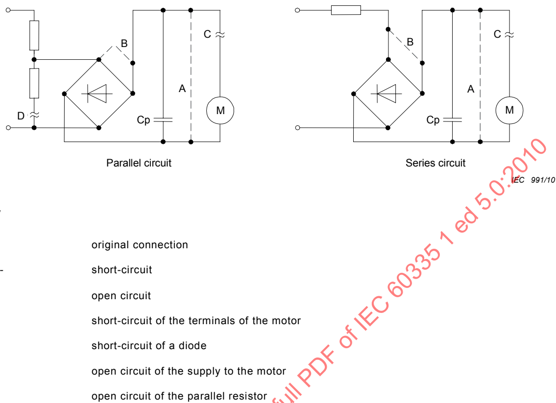
Figure I.1 – Simulation of faults
