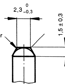
Permissible variation for the end of pins
