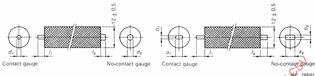
Gauge for 0,2 A and 2,5 A connectors
