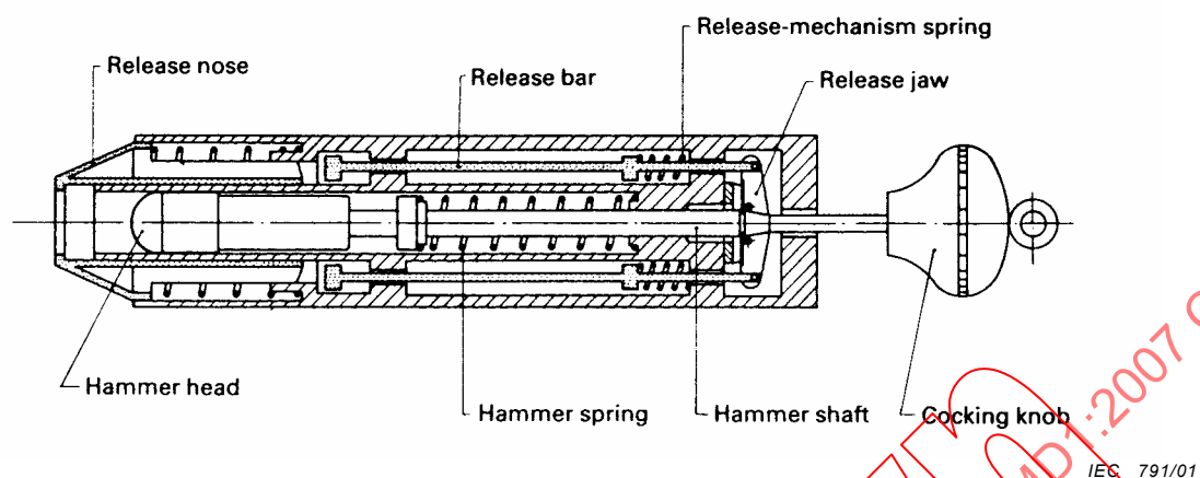
Figure 21 – Impact-test apparatus (see 23.5)
