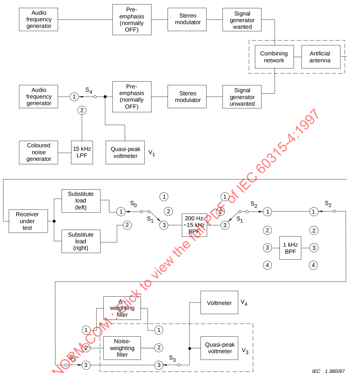
Figure 6 – Arrangement for various measurements with two r.f. input signals
