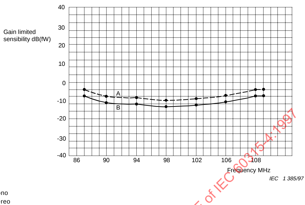
Figure 11 – Gain-limited sensitivity as a function of signal frequency
