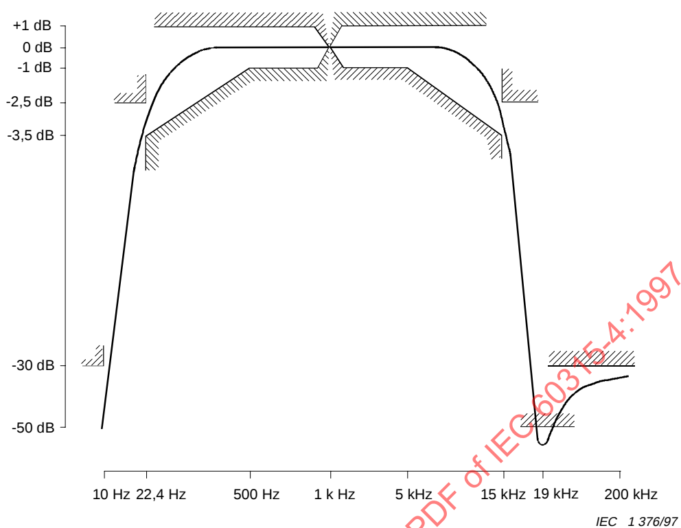
Figure 2 – Frequency response limits of band-pass filter 22,4 Hz to 15 kHz
