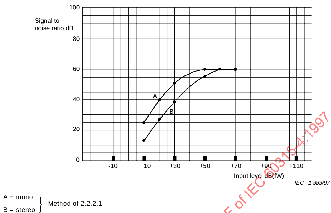
Figure 9 – Signal-to-noise ratio
