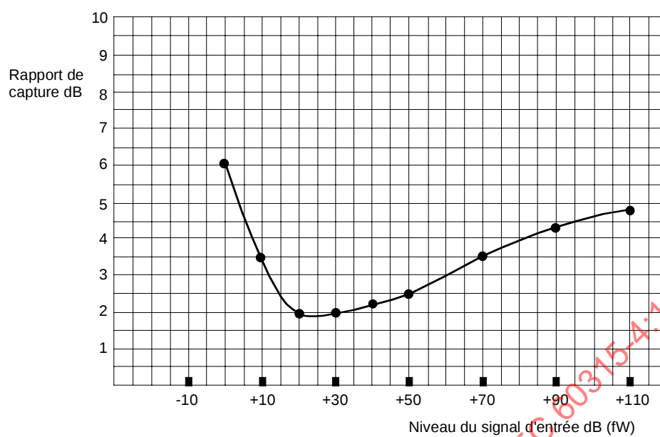
Figure 13 – Rapport de capture
