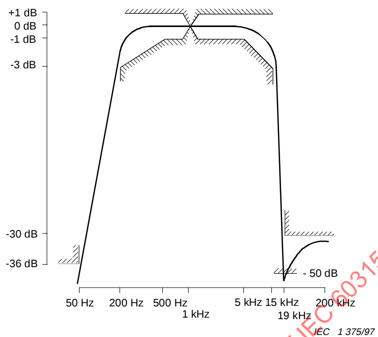
Figure 1 – Frequency response limits of band-pass filter 200 Hz to 15 kHz
