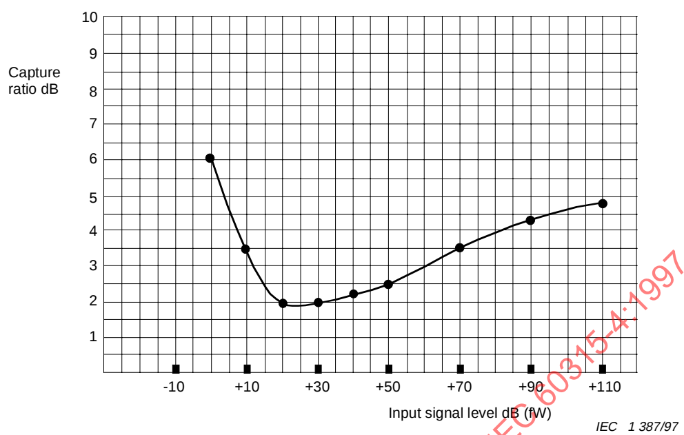
Figure 13 – Capture ratio
