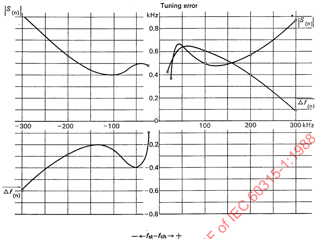
FIG. 9. — Mean tuning error and its standard deviation of a push-button tuning system, as functions of the difference between the frequency of the starting position, f_{st} , and the chosen operating frequency, f_{ch} , of 1.0 MHz and for n = 10 measurements (see Sub-clause 26.3).
