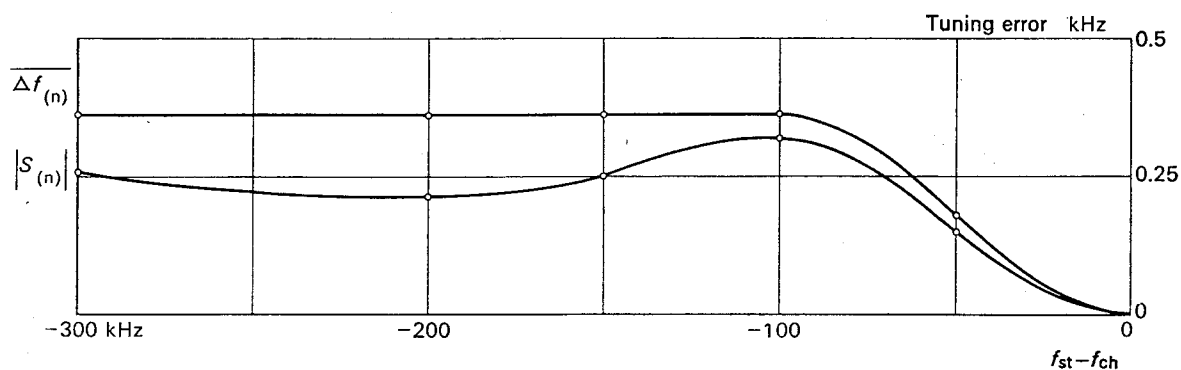
FIG. 11. — Mean tuning error and its standard deviation for an automatic search system, as functions of the frequency difference between the starting position and the stop signal, for f_{\text{stop}} = 1.4 MHz at an input signal level of 60 dB ( \mu\text{V} ) and n = 10 measurements (see Sub-clause 27.3).
