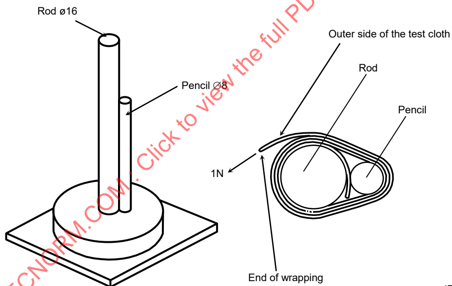
Figure 6 – Wrapping rod and pencil
