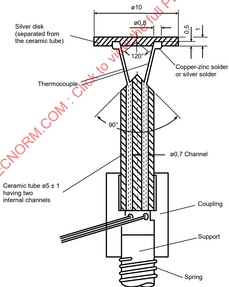
Figure 1 – Arrangement for measuring the sole-plate temperature
