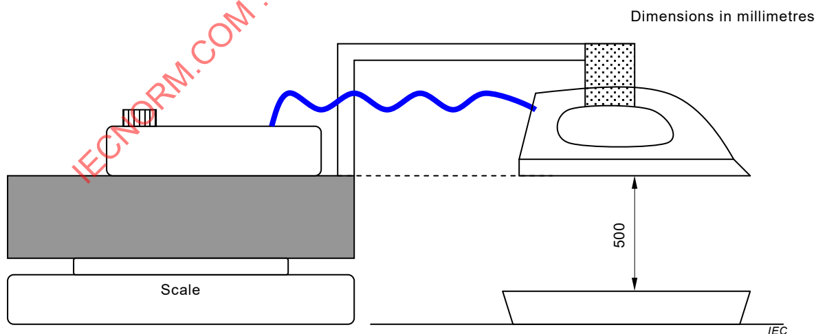
b) – Pressurized or instantaneous steam irons
