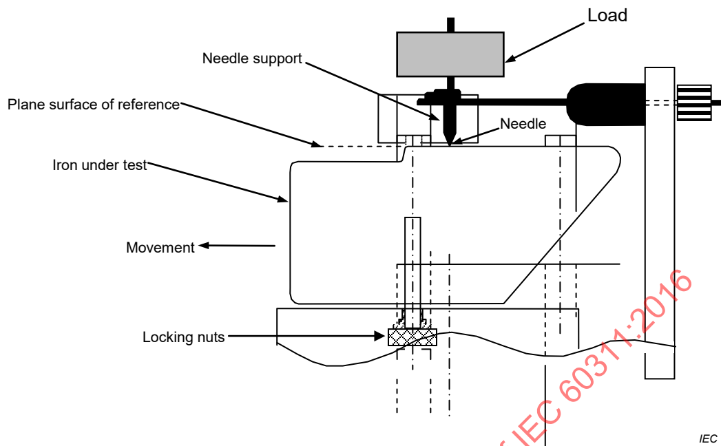
a) – Test apparatus for scratch resistance of sole-plate
