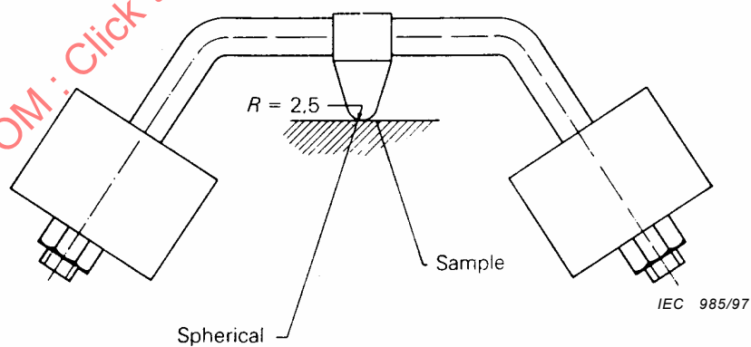
Figure 10 – Ball-pressure apparatus
