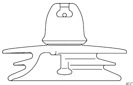
Figure 5 – Profil type "à trois ailettes externes" "T"
