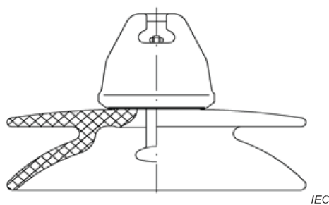
Figure 4 – Profil type "à deux ailettes externes" "V"
