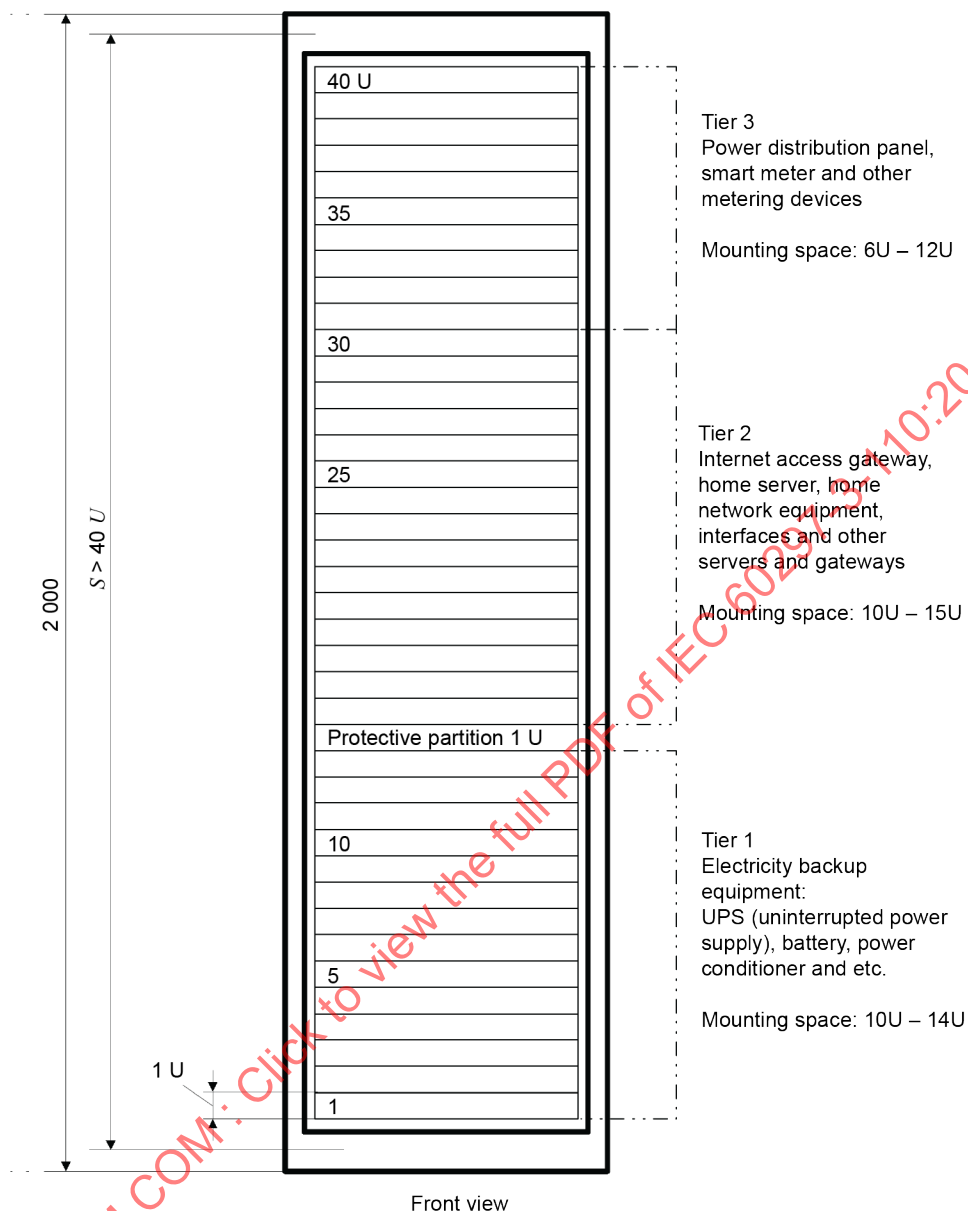
Figure 5 – Typical equipment categories and their mounting locations of a 2 000 mm high (40U) residential rack or cabinet
